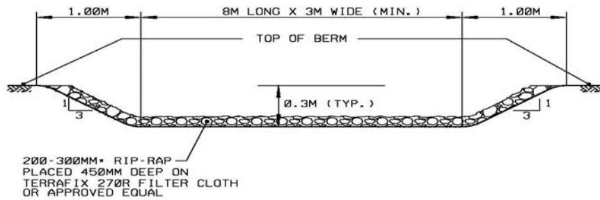
SECTION B-B EMERGENCY WEIR
