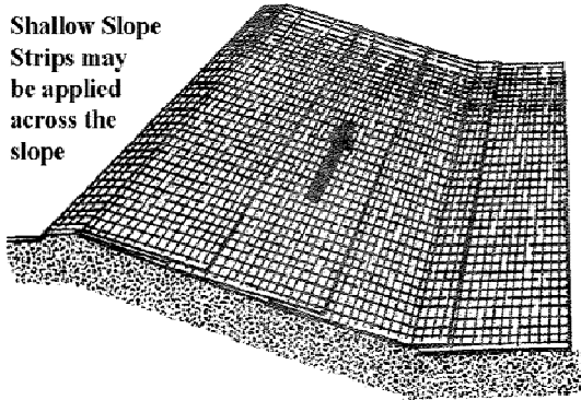
Figures illustrating the installation of erosion control mats, blankets, and nets from Keeping Soil on Construction Sites (HRCA & HCA, 1994).
