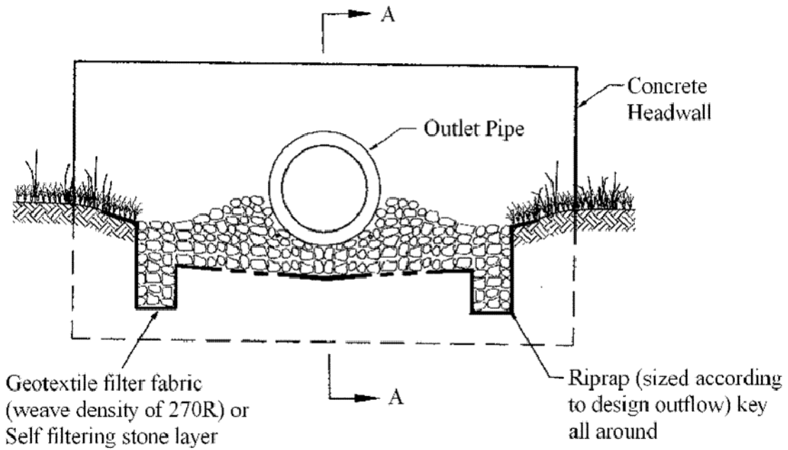
Figures illustrating a storm drain outfall protection from Sediment & Erosion Control on Construction Sites – Field Guide (University of Virgin Islands, 2003)
