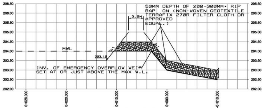
SECTION C-C EMERGENCY WEIR PROFILE
